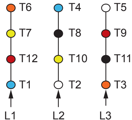
LOW VOLTAGE (ΔΔ)
