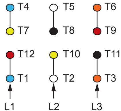
HIGH VOLTAGE (Δ)
