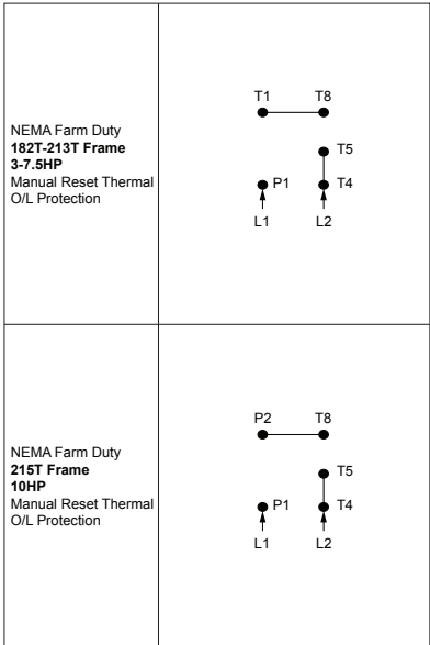
208-230V 60Hz Direct-on-line (DOL) full voltage starting
