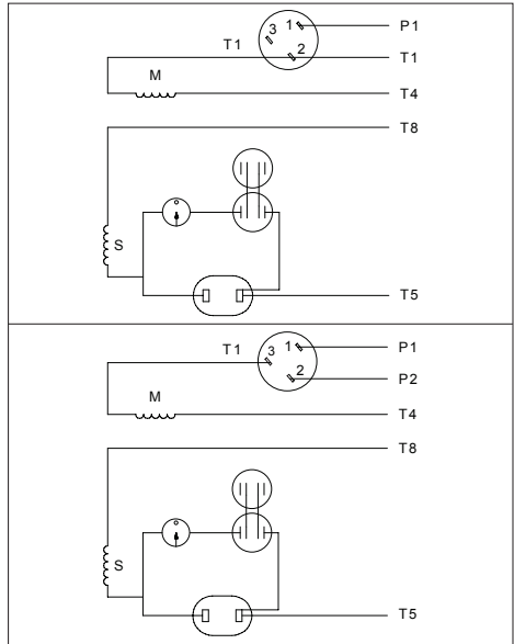
Thermally Protected Single-Phase Circuit Diagram
